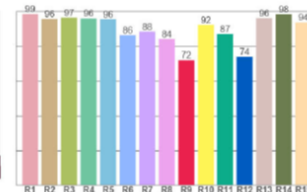
CRI: 92.6 (R1-R8)
